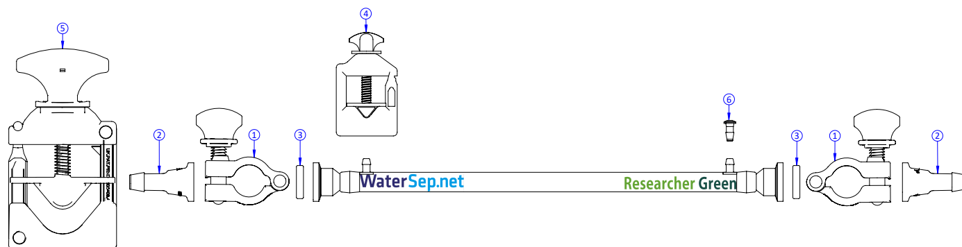
Diagram: FlowConnector™ Kit- Researcher™ without sensors
