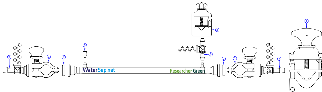
Diagram: Flow Connector Kit- Researcher™ with sensors
