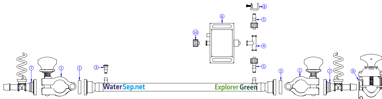
Diagram: FlowConnector™ Kit- Explorer™ with sensors
