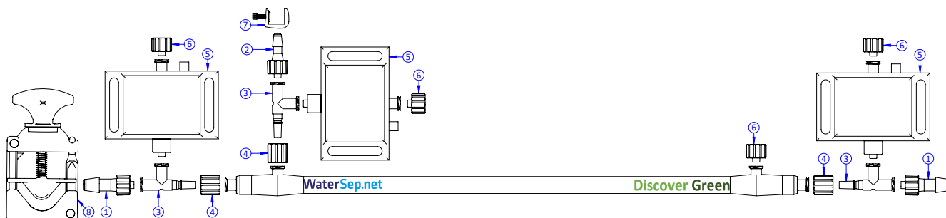
Diagram: FlowConnector ™ Kit- Discover ™ with sensors
