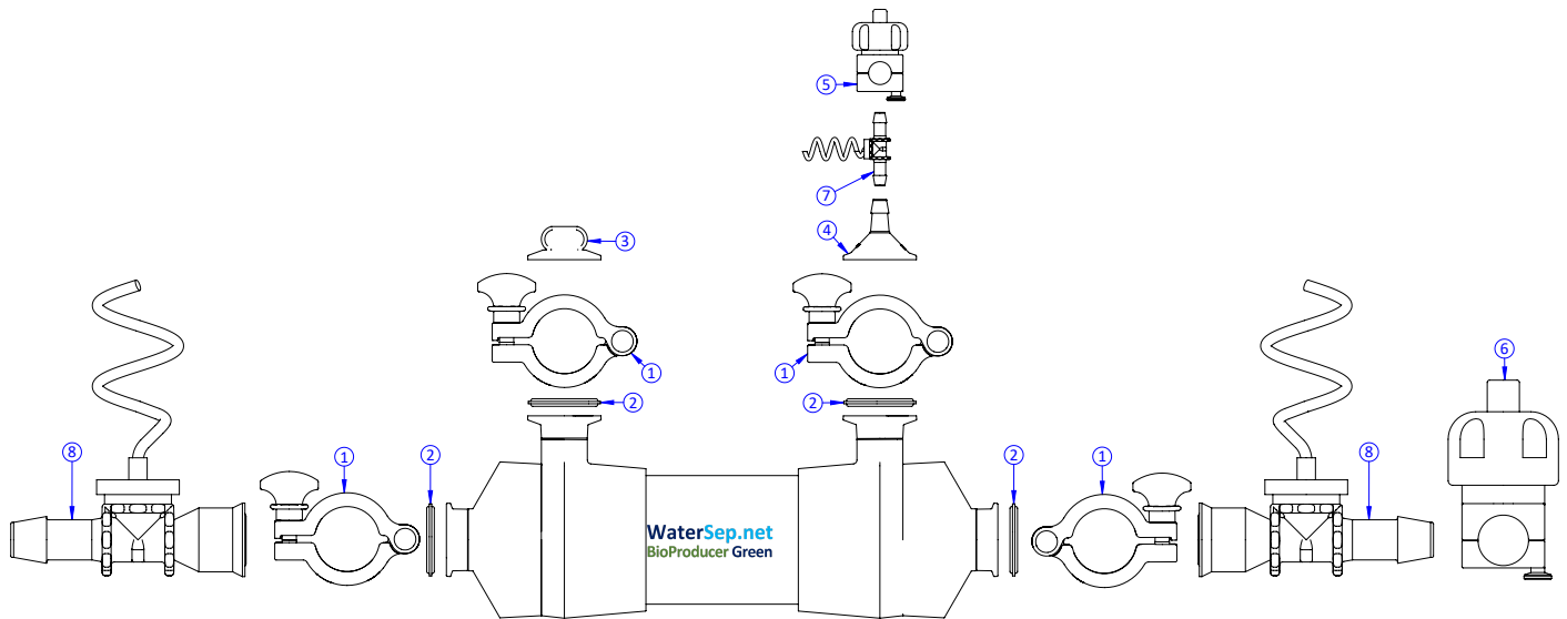
Diagram: FlowConnector™ Kit- BioProducer™ with sensors
